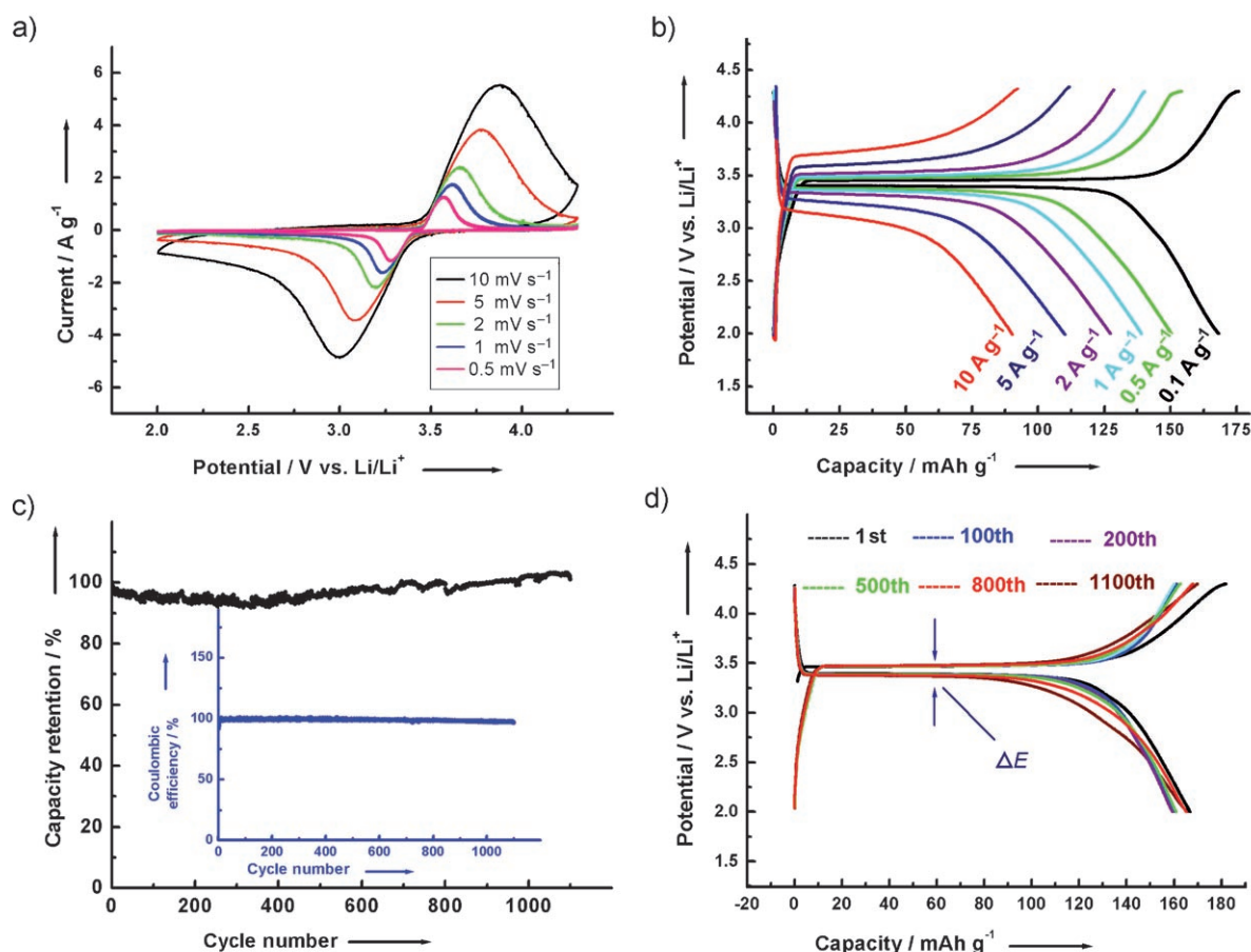
Figure 4. Electrochemical characterization of the prepared \text{LiFePO}_4/\text{carbon} composite: a) Cyclic voltammetry tests at different scan rates in the potential window 2.0–4.3 V (vs. \text{Li}/\text{Li}^+ ); b) charge–discharge tests at different current densities in the potential window 2.0–4.3 V (vs. \text{Li}/\text{Li}^+ ); c) cycling profile tested at a current density of 0.1 \text{ A g}^{-1} between 2.0 and 4.3 V; d) charge–discharge curves at different cycle number.
